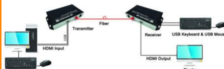
HK-HDMI-KVM
